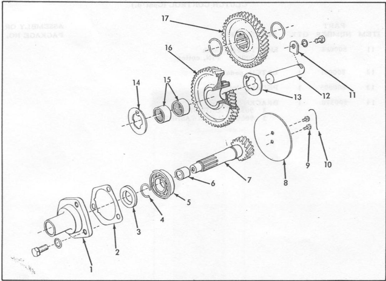
CLUTCH SHAFT & INTERMEDIATE GEARS
