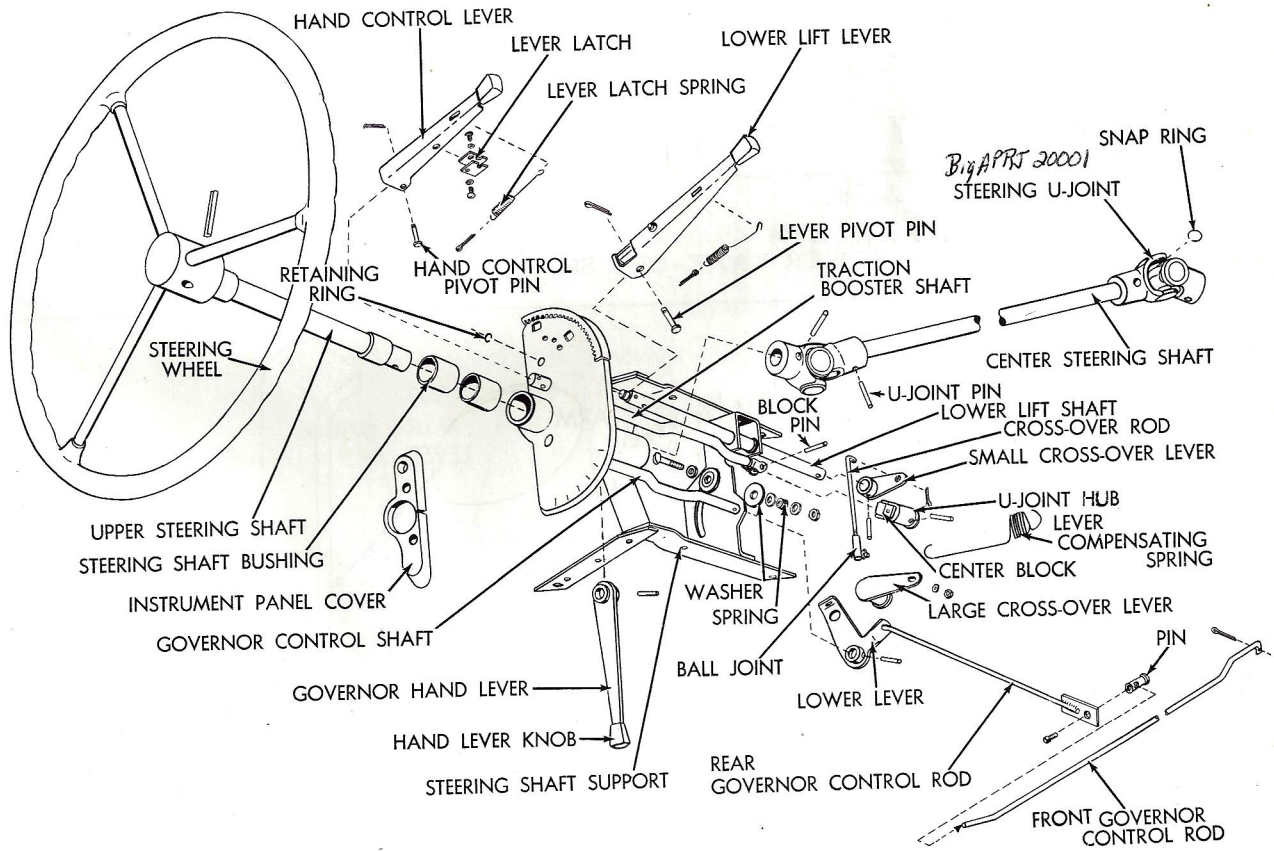
STEERING SHAFT SUPPORT & HAND CONTROLS
