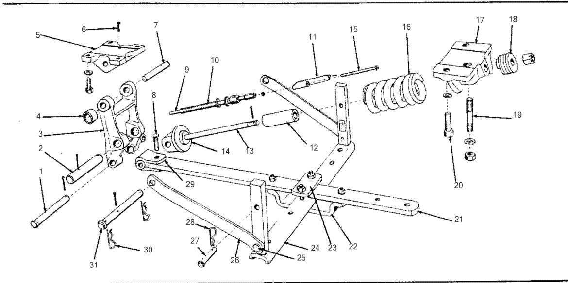
DRAWBAR HITCH
